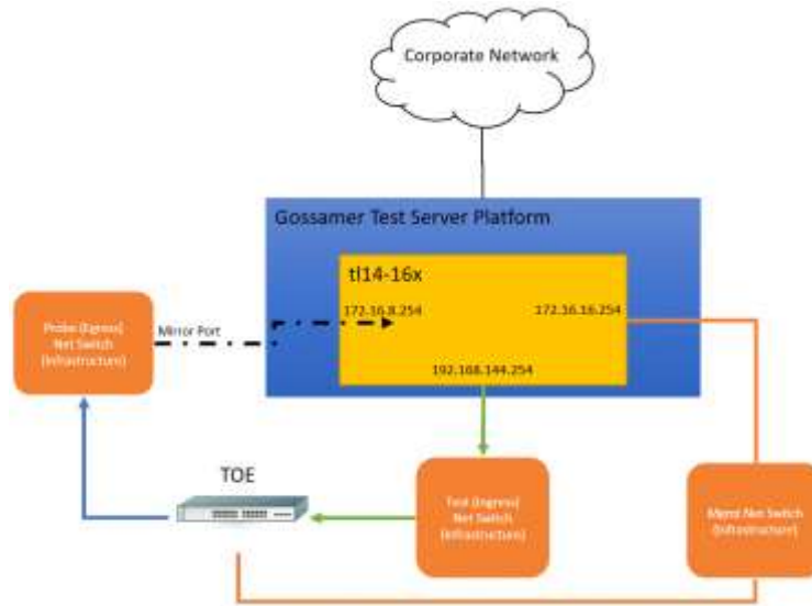
Figure 1 Test Setup
