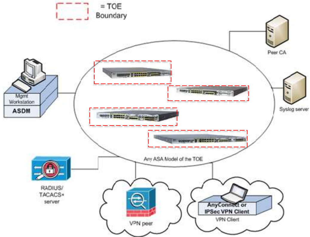
Figure 2: Example of TOE Deployment
