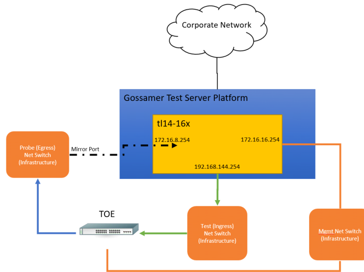
Figure 1 Test Setup
