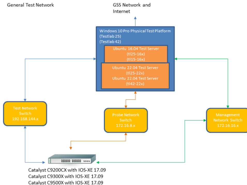
Figure 1 Test Setup
