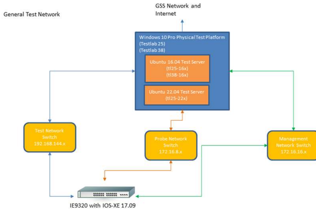
Figure 1 Test Setup
